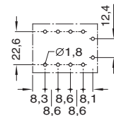
Hole pattern for solder pin connections
