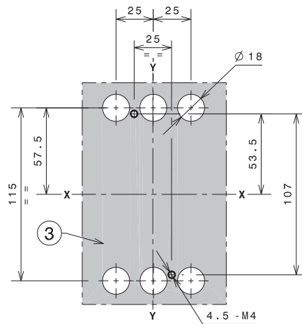
3 POLES
