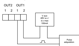
Digital output used as pulses
