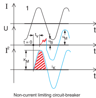
Oscillogram of short-circuit breaks on two circuit-breakers:
