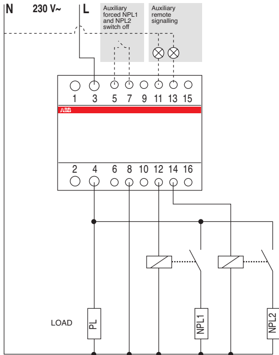
Single-phase wiring diagram for non-priority loads with 16 A or more current consumption
