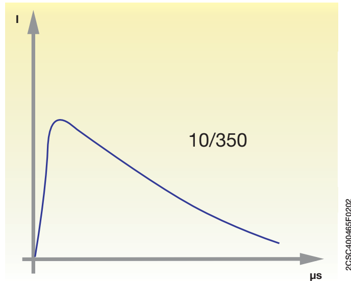
Type 1 Surge Arresters I_{imp} : current wave
