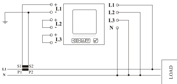
Single phase insertion with 1CT
