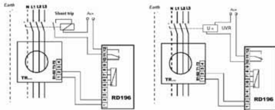
Example of wiring diagram: shunt trip connection and undervoltage release (fail safe OFF)
