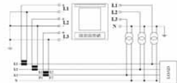
4 wires insertion
