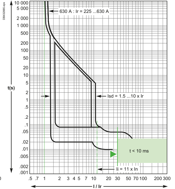
MicroLogic 2.3, 4.3 - 630 A
