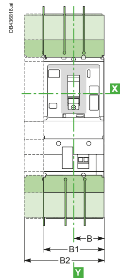
NSX100 to 630 [2]
