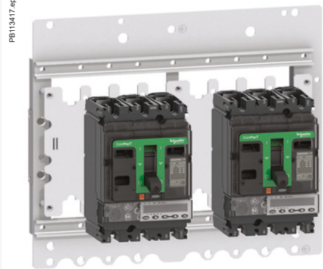
Interlocking on a base plate
