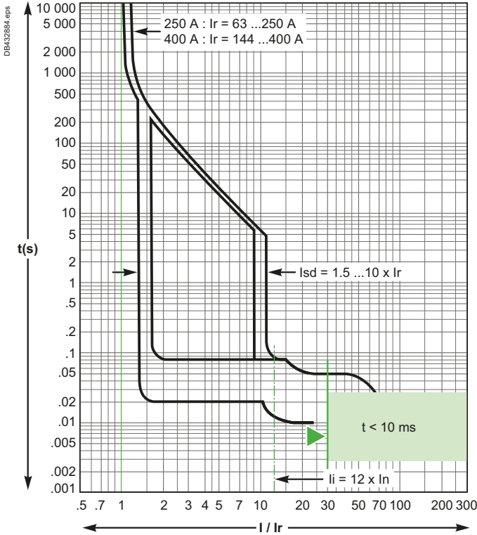
MicroLogic 2.3, 4.3 - 250... 400 A
