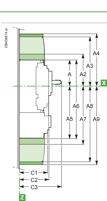
NSX100 to 250
